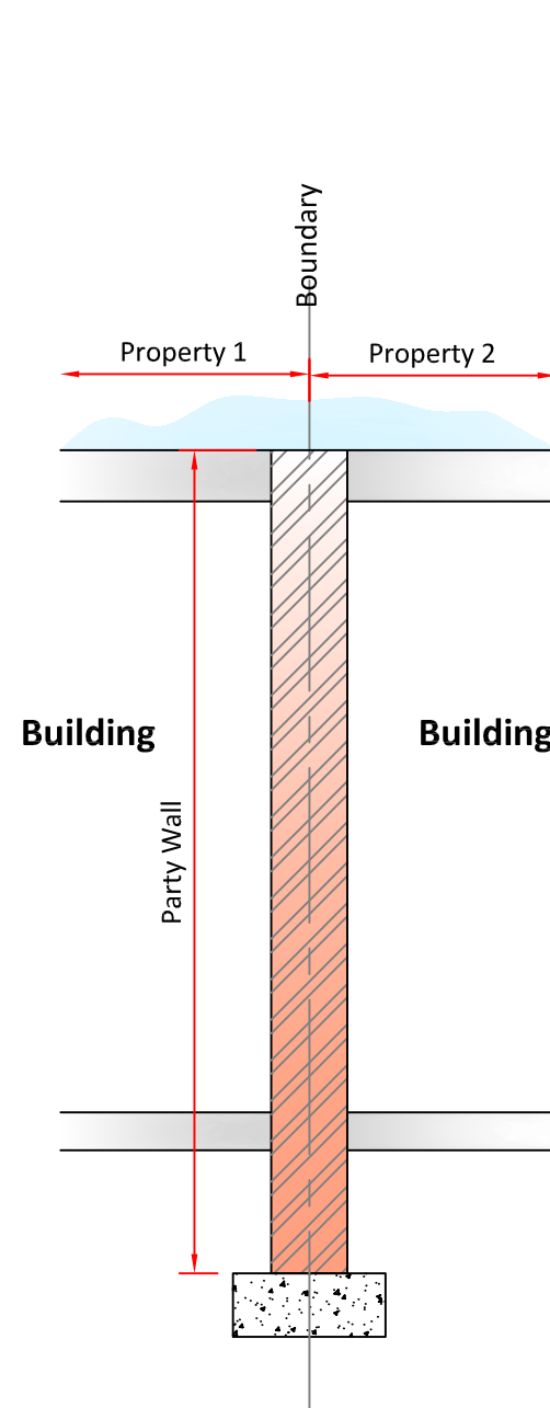
PARTY WALL TYPE A
