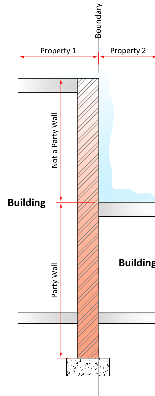
PARTY WALL TYPE B
