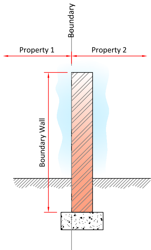
BOUNDARY WALL
